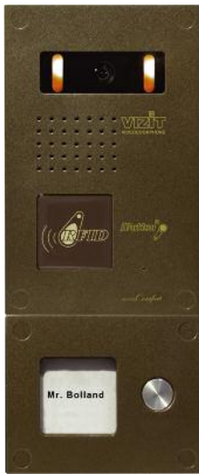
BS-1 95x75x9.5 -30...+45°C surface-mounted
